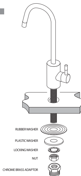
TAP INSTALL DIAGRAM
